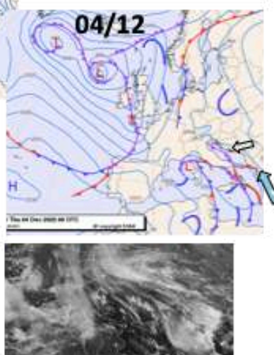
c - Meteosat
